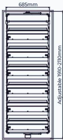
FRONT VIEW Unit Dimensions
